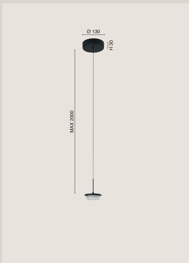
▲ Tonda 1 luce 1 Light round 14W - 1510lm
